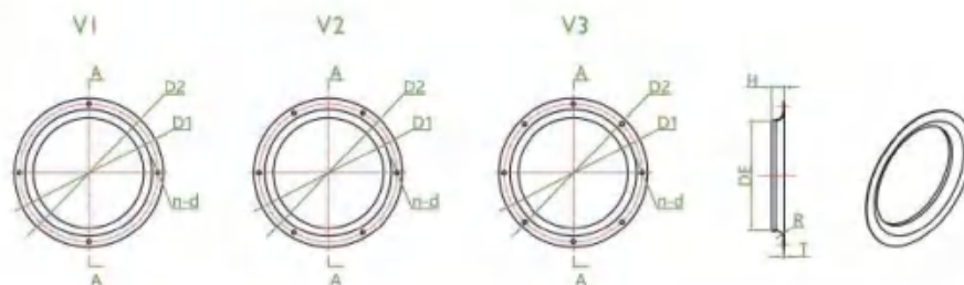
Inlet Rings for Backward Curved Centrifugal Fans
